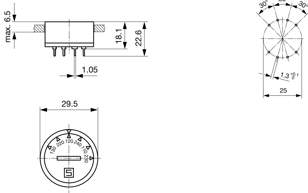
Dimension 29.5 mm Drilling diagram
