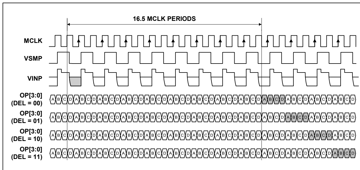
Figure 32 Mode 3 Operation
