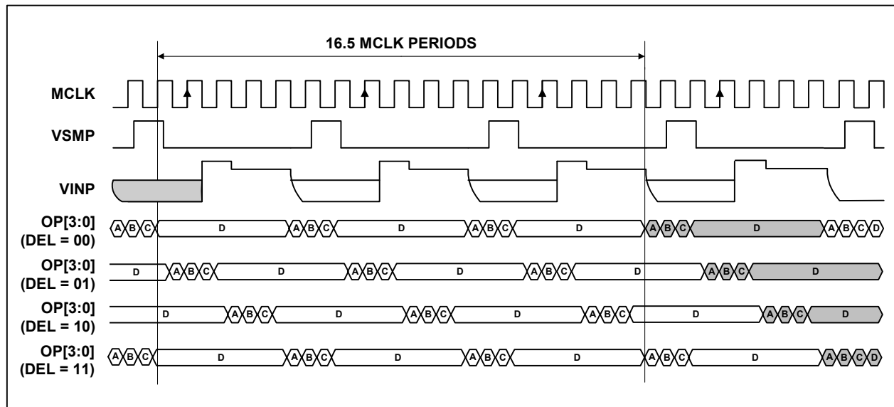
Figure 30 Mode 1 Operation
