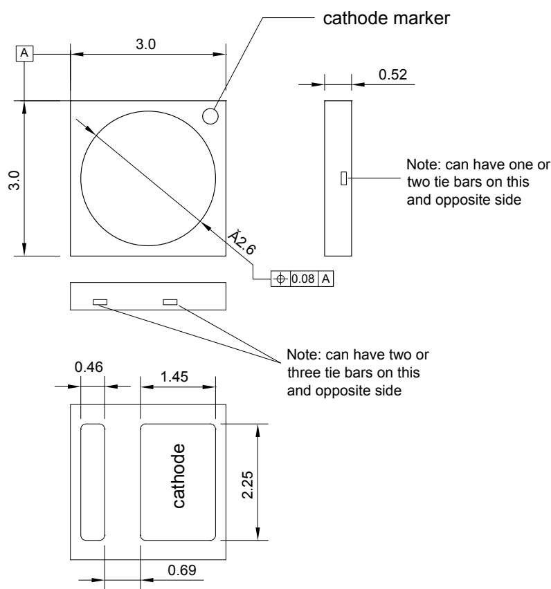
Figure 13: Mechanical dimensions for LUXEON 3030 2D.
