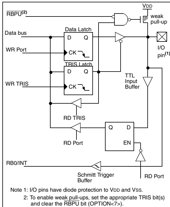
FIGURE 3-3: BLOCK DIAGRAM OF BB3:BB0 PINS
