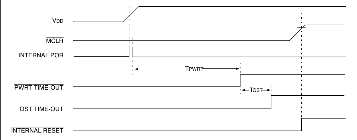
FIGURE 10-9: TIME-OUT SEQUENCE ON POWER-UP ( \overline{\text{MCLR}} NOT TIED TO \text{V}_{\text{DD}} ): CASE 2
