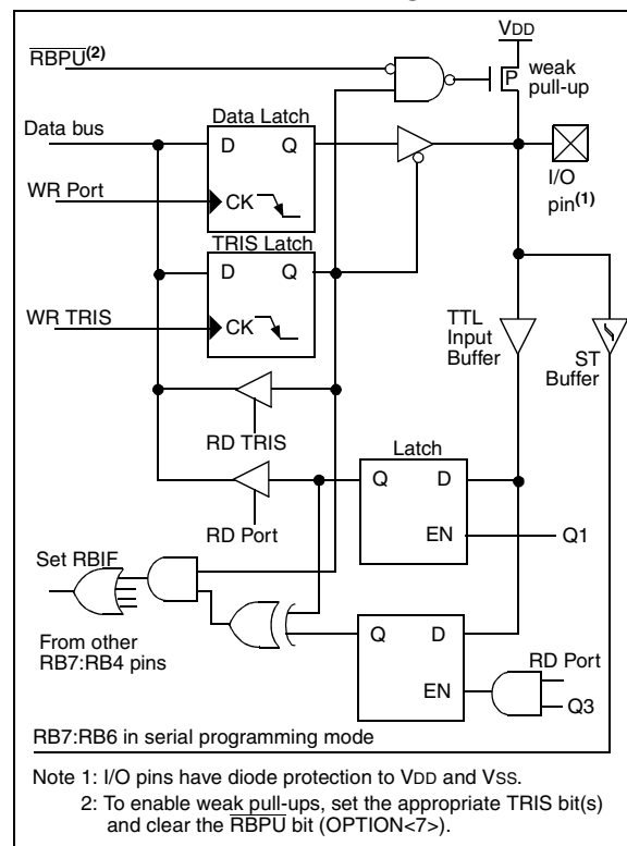
FIGURE 3-4: BLOCK DIAGRAM OF BB7:BB4 PINS
