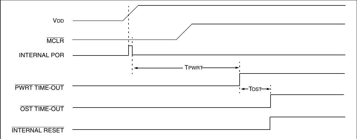
FIGURE 10-8: TIME-OUT SEQUENCE ON POWER-UP ( \overline{\text{MCLR}} NOT TIED TO \text{V}_{\text{DD}} ): CASE 1
