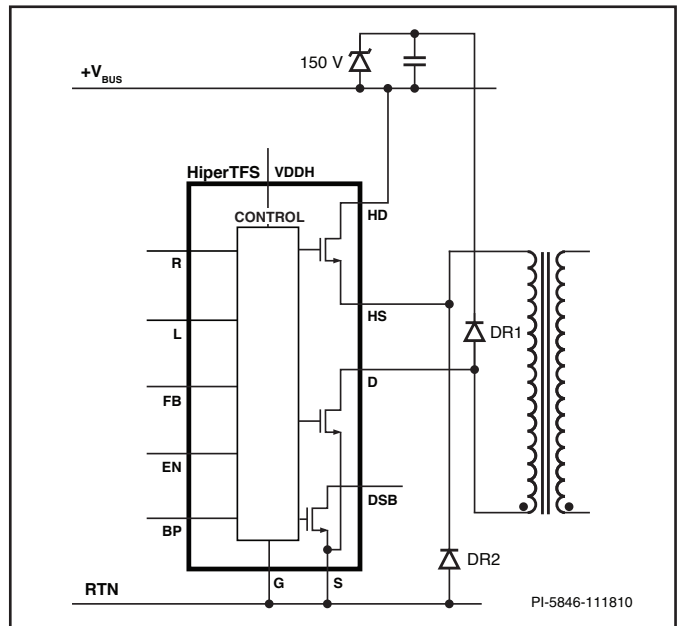
Figure 15. Typical Primary Winding Clamp-to-Rail.
