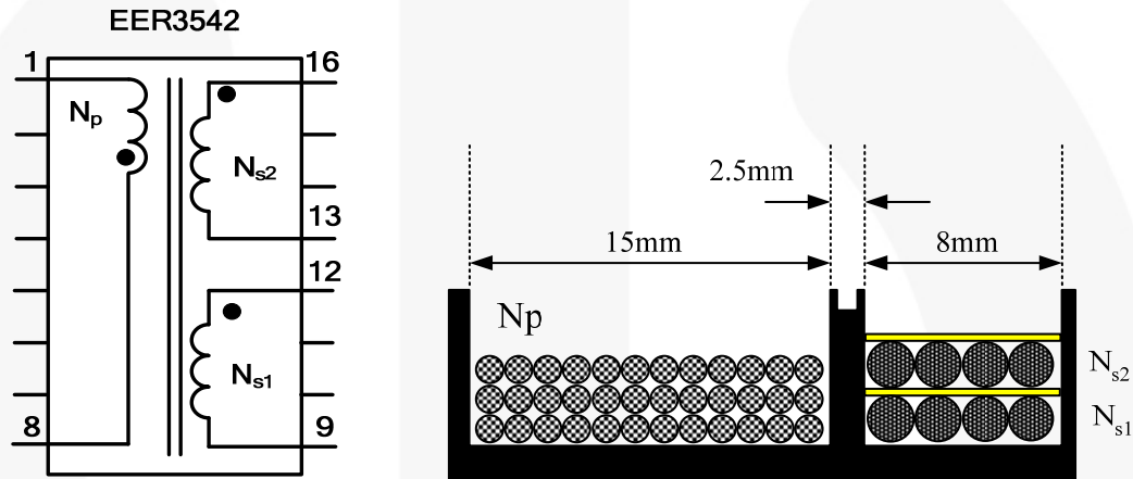
Figure 5. Transformer specification.
