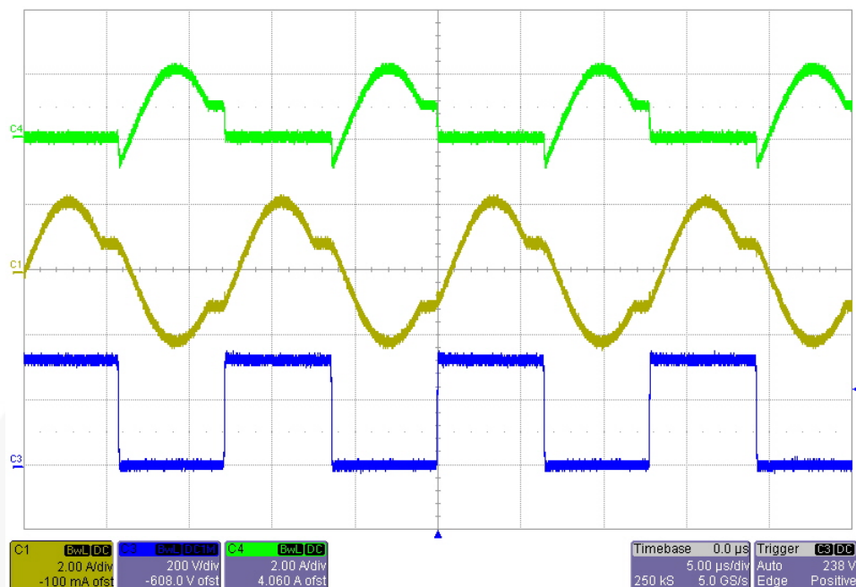
Figure 10. Operation Waveforms at Minimum Input Voltage [ V_{IN}=340V_{DC} , P_O=192W (24V/8A)]; C4: Transformer Primary-Side Current (2A/div); C1: Low-Side MOSFET Current (2A/div); C3: Low-Side MOSFET V_{DS} (200V/div), Time: 5μs/div
