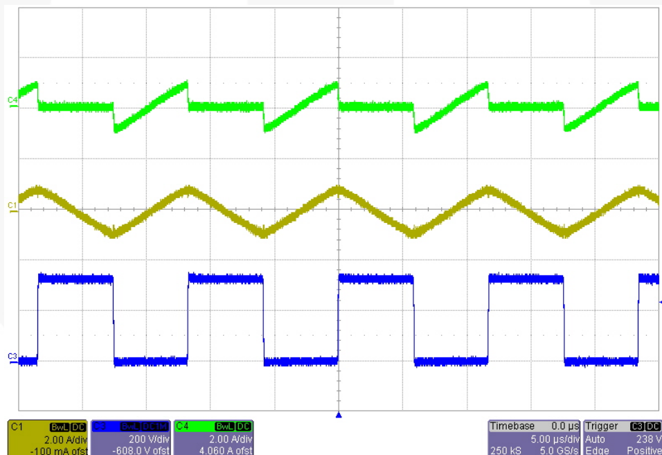
Figure 11. Operation Waveforms at Minimum Input Voltage [ V_{IN}=340V_{DC} , P_O=0W (24V/0A)]; C4: Transformer Primary-Side Current (2A/div); C1: Low-Side MOSFET Current (2A/div); C3: Low-Side MOSFET V_{DS} (200V/div), Time: 5μs/div
