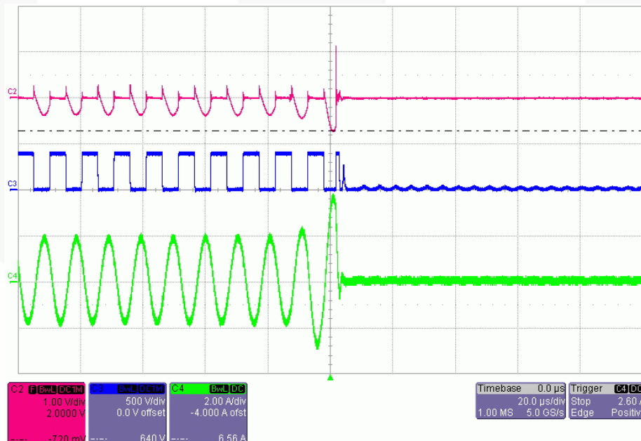
Figure 24. Protection Waveform at Output Short Condition [ V_{IN}=390V_{DC} , ( I_O=8A \rightarrow \text{Short} )]; C2: Current Sensing Pin (CS) Voltage (1V/div); C3: Low-Side MOSFET V_{DS} (500V/div); C4: Transformer Primary-Side Current (2A/div), Time: 20μs/div
