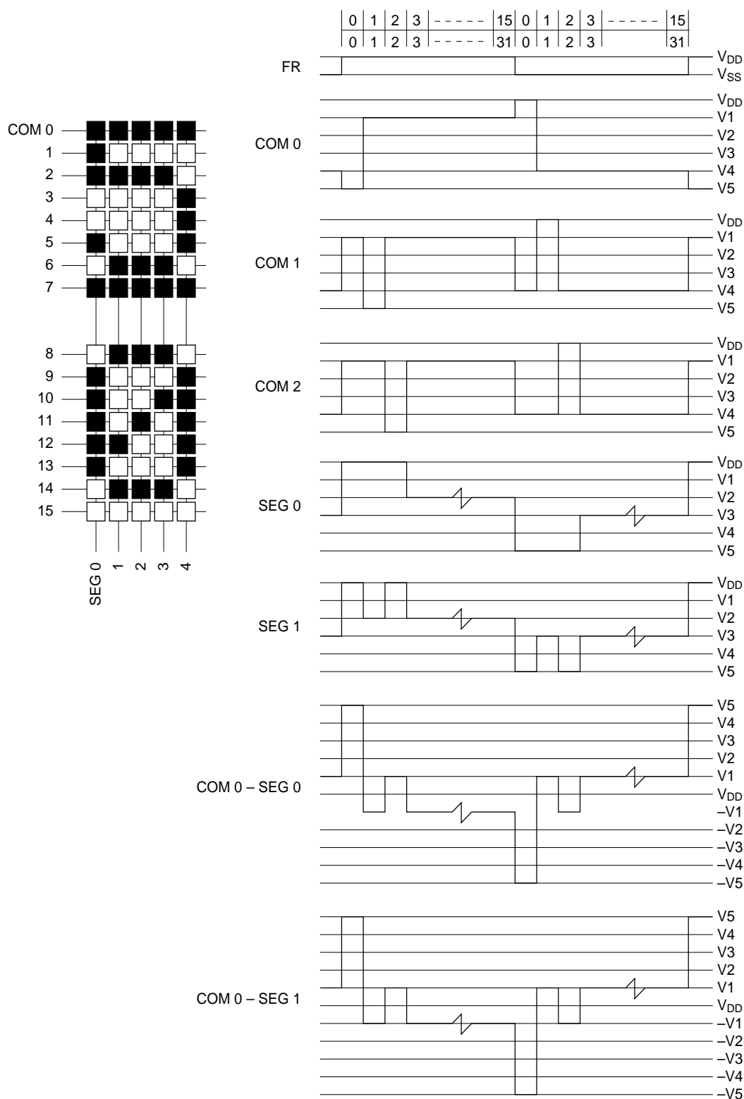
Figure 3.6. Examples of LCD Driving Waveform
