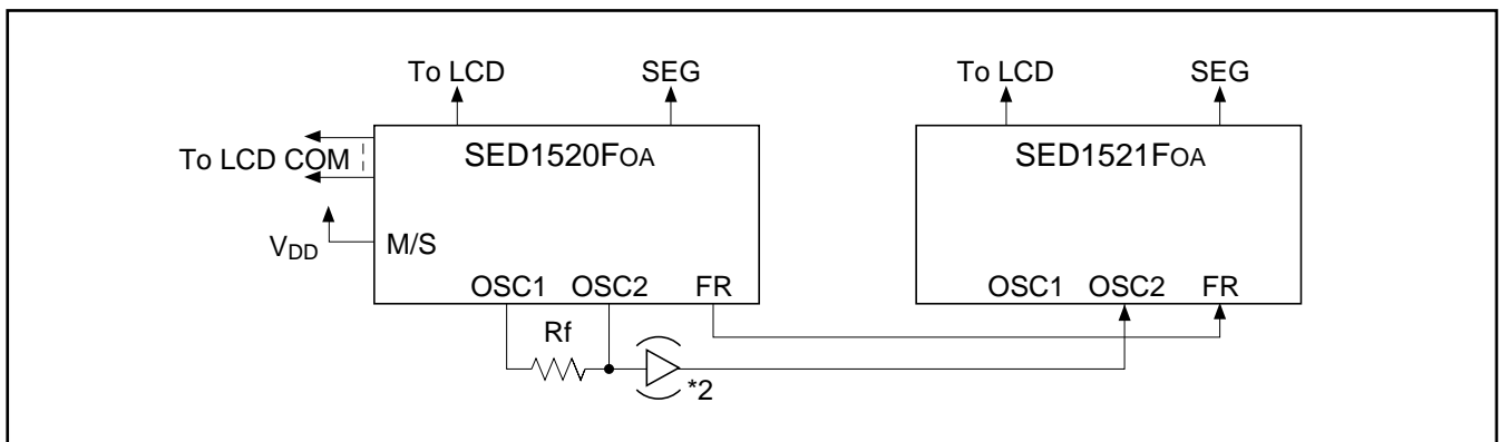
Figure 7.3 SED1520FOA – SED1521FOA *1
