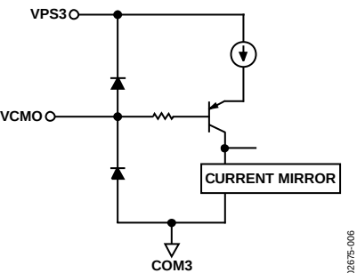
Figure 38. Circuit C
