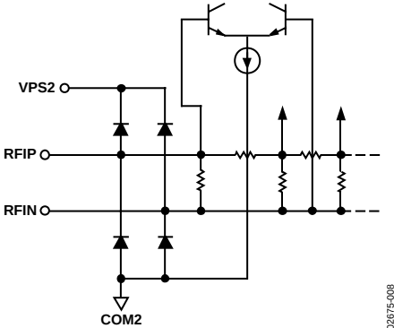
Figure 40. Circuit E
