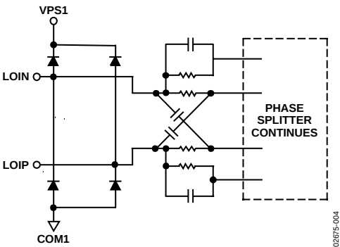
Figure 36. Circuit A
