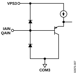
Figure 39. Circuit D
