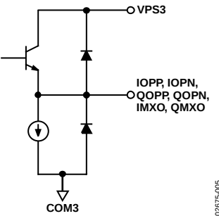
Figure 37. Circuit B
