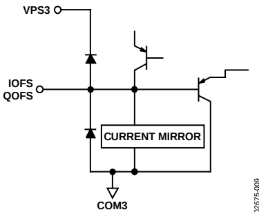
Figure 41. Circuit F
