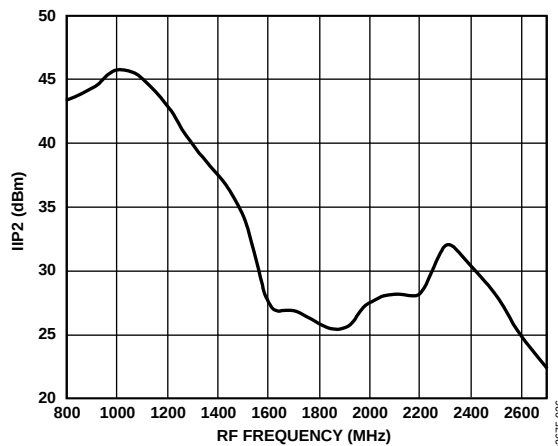
Figure 17. IIP2 vs. F_{LO} , V_{VGIN} = 1.2 V, Baseband Tone1 = 5 MHz, -10 dBm, Baseband Tone2 = 6 MHz, -10 dBm, Temperature = 25°C, V_S = 5 V
