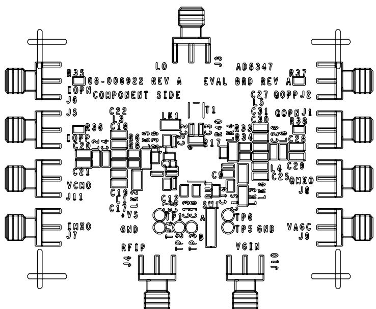
Figure 54. Silkscreen of Component Side
