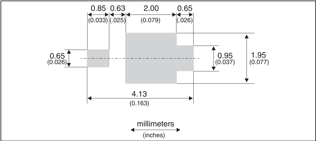
Figure 21. Footprint dimensions
