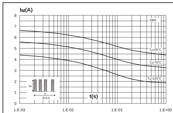
Figure 7. Non repetitive surge peak forward current versus overload duration - maximum values
