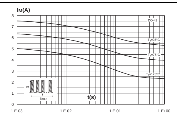
Figure 8. Non repetitive surge peak forward current versus overload duration - maximum values
