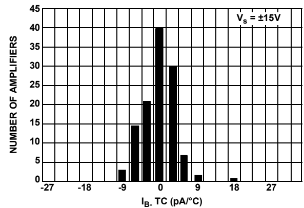
FIGURE 19. I_{B-} INPUT BIAS CURRENT DRIFT DISTRIBUTION, V_S = \pm 15V
