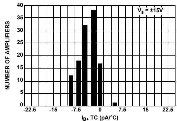
FIGURE 17. I_{B+} INPUT BIAS CURRENT DRIFT DISTRIBUTION, V_S = \pm 15V
