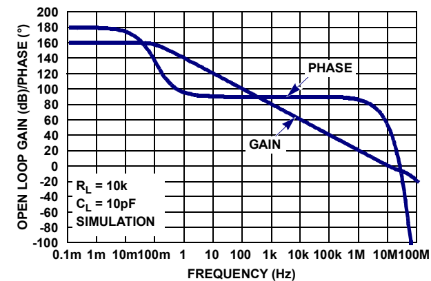
FIGURE 55. SIMULATED OPEN-LOOP GAIN, PHASE vs FREQUENCY
