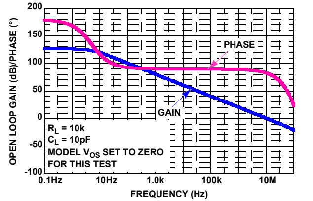
FIGURE 56. SIMULATED OPEN-LOOP GAIN, PHASE vs FREQUENCY
