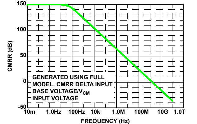
FIGURE 58. SIMULATED CMRR vs FREQUENCY
