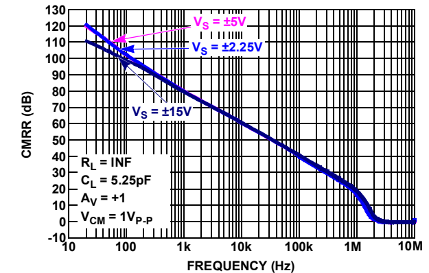
FIGURE 57. CHARACTERIZED CMRR vs FREQUENCY
