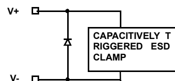
CIRCUIT 3
