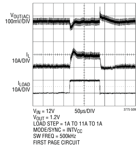
Load Step in Pulse-Skipping Mode
