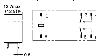
Terminal Arrangement/ Internal Connection (Bottom View)
