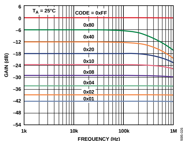
Figure 25. Gain vs. Frequency vs. Code, R_{\text{AB}} = 20 \text{ k}\Omega
