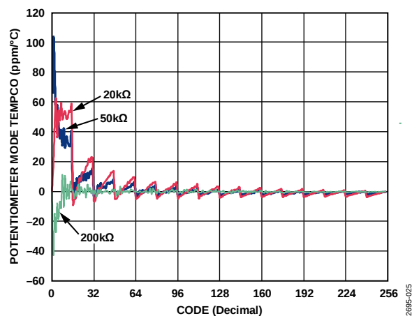
Figure 24. Potentiometer Mode Tempco \Delta V_{\text{WB}}/\Delta T vs. Code
