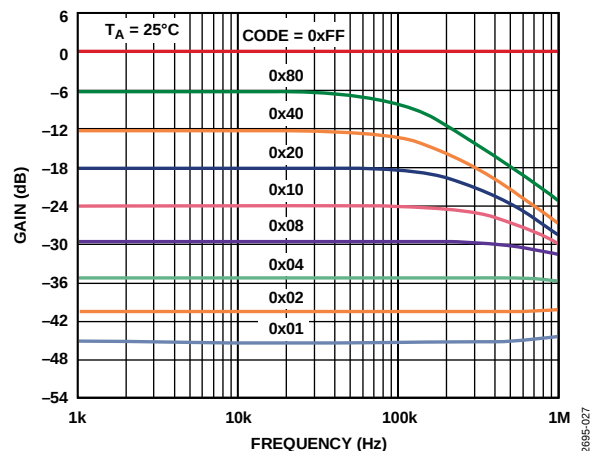
Figure 26. Gain vs. Frequency vs. Code, R_{\text{AB}} = 50 \text{ k}\Omega
