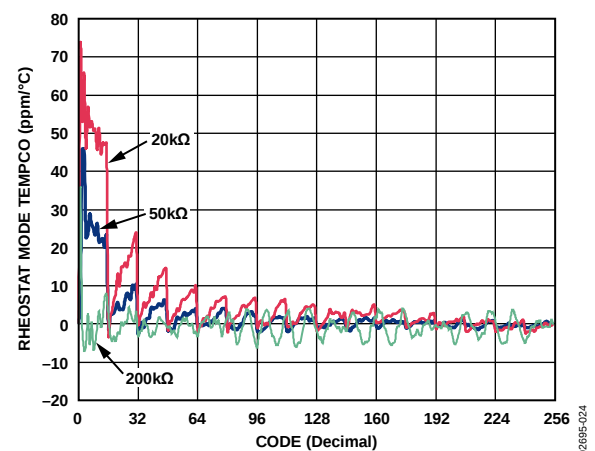
Figure 23. Rheostat Mode Tempco \Delta R_{\text{WB}}/\Delta T vs. Code
