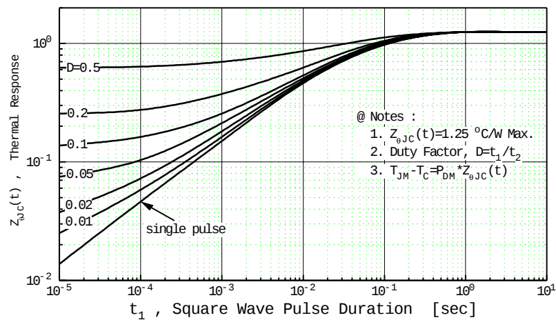
Figure 11. Thermal Response
