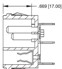
Cross Section
