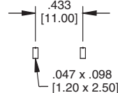
Recommended Panel Cut-Out
