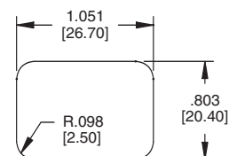
Recommended Panel Thickness: 0.80mm - 3.0mm
