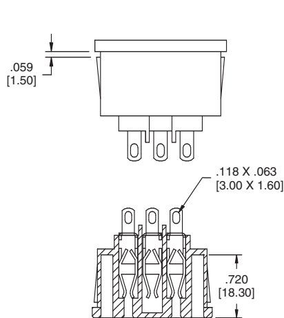
Cross Section
