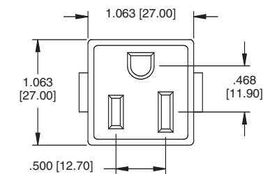
Recommended Panel Cut-Out For 1.50mm Panel Thickness
