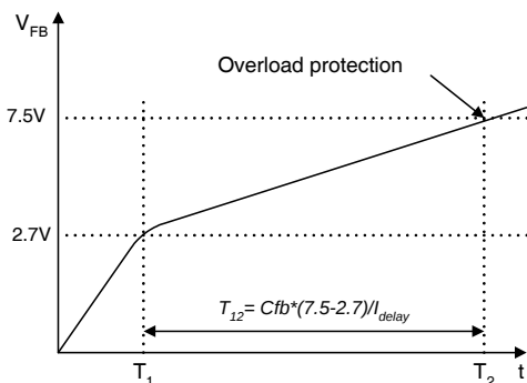
Figure 27. Overload protection
