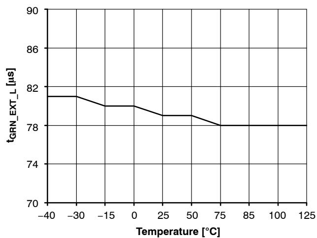
Figure 16. t_{GRN\_EXT\_L}
