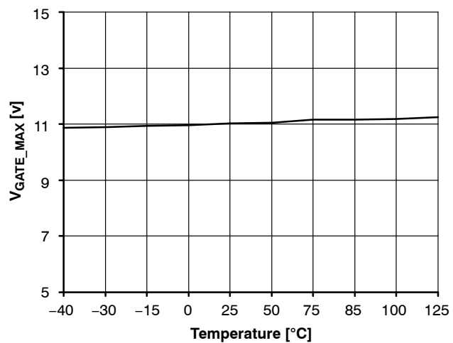
Figure 18. V_{GATE\_MAX}
