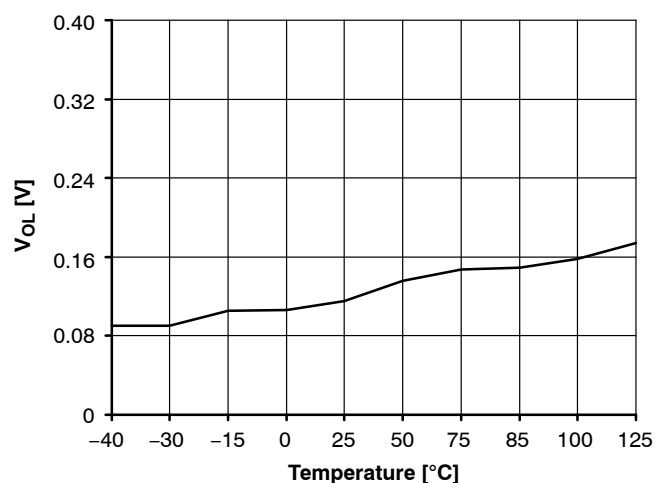
Figure 20. V_{OL}
