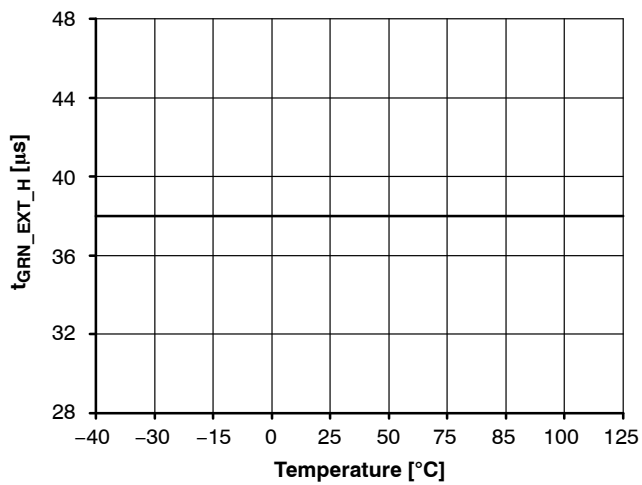
Figure 15. t_{GRN\_EXT\_H}
