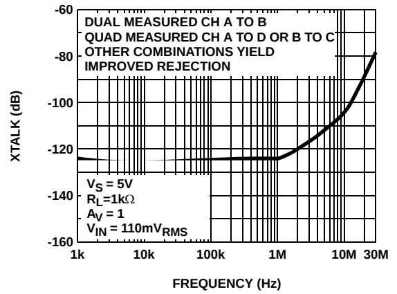
FIGURE 20. CHANNEL SEPARATION
