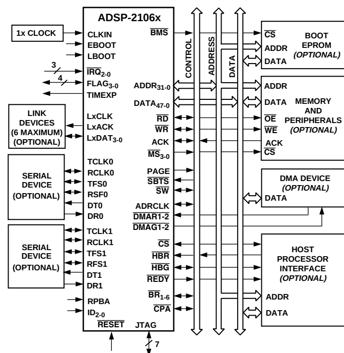
Figure 2. ADSP-21062 System
