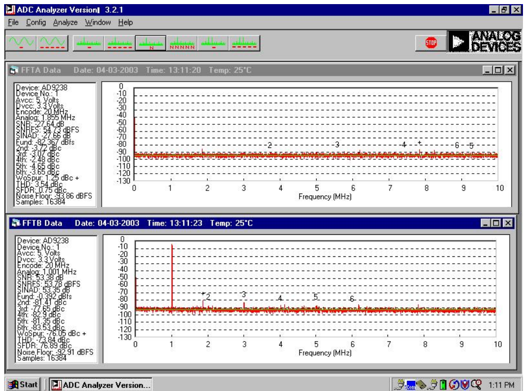
Figure 13. FFT, Channel 2
