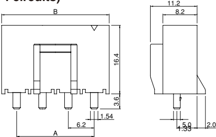
(Single-row 4 circuits)
