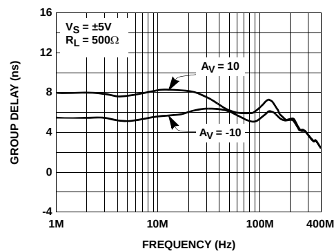
FIGURE 28. GROUP DELAY vs FREQUENCY
