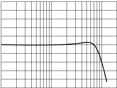
FIGURE 5. NON-INVERTING FREQUENCY RESPONSE FOR VARIOUS GAIN
