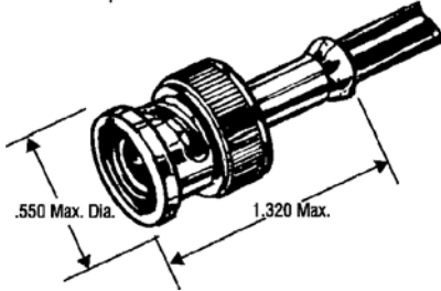
Hex Crimp
