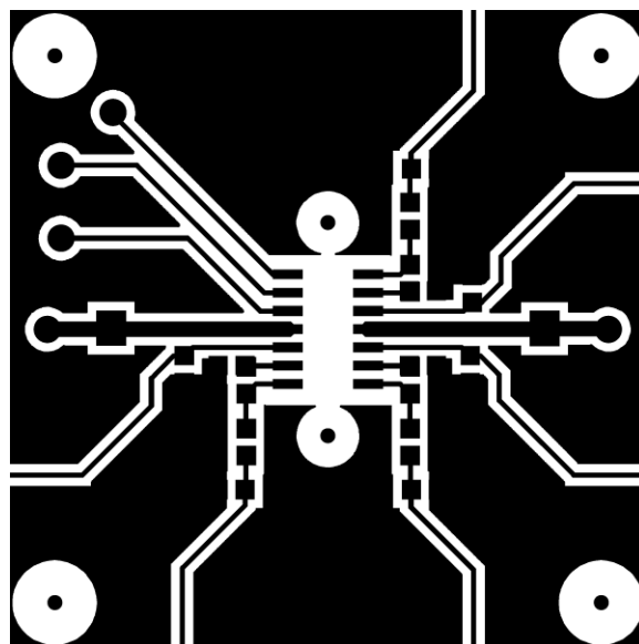
Figure 5. Board Layout Pattern, Circuit Side
