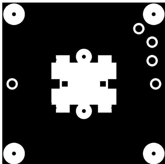
Figure 4. Board Layout Pattern, Component Side
