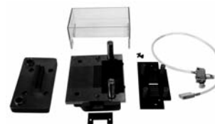
Ribbon Cable Notcher Assembly
