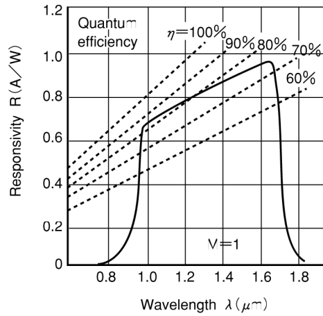
Fig.1 Spectral response
