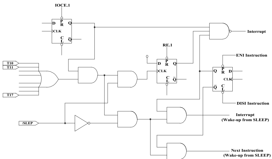
Fig. 8 The circuit of I/O port and I/O control register for P61~P67
