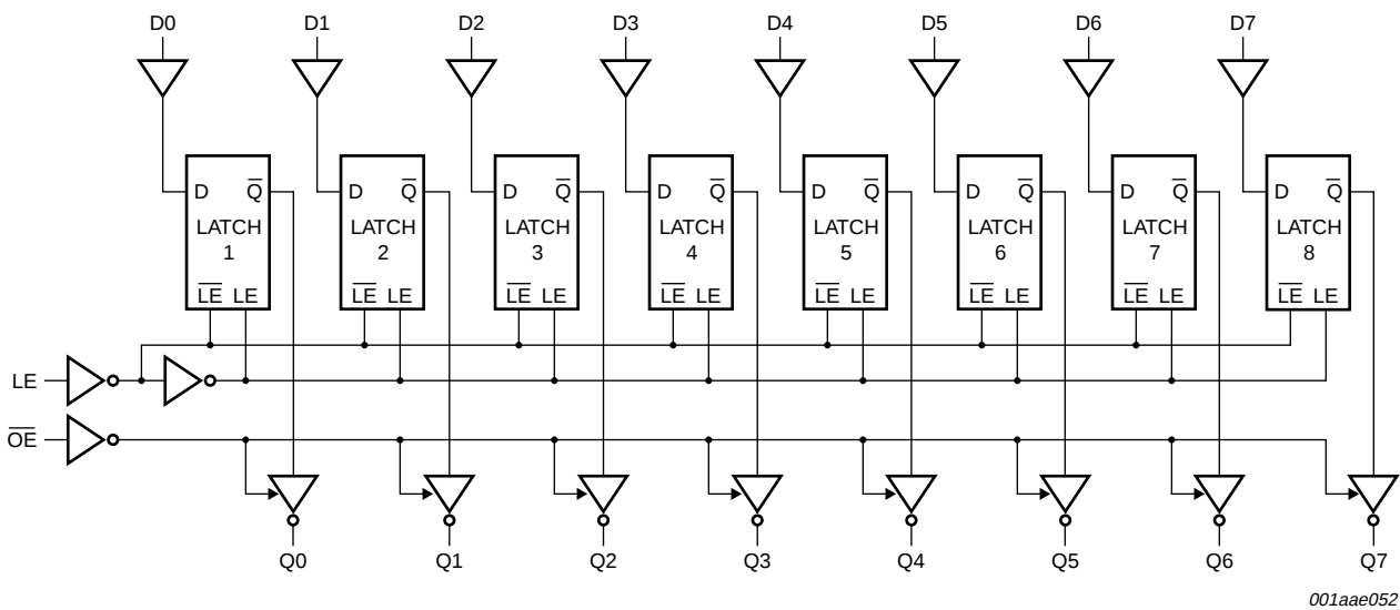
Fig 4. Logic diagram
