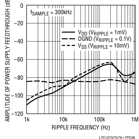
Power Supply Feedthrough vs Ripple Frequency (LTC1275/76)
