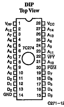
Figure 1. Programming Pinouts
