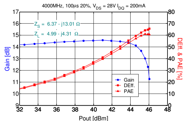
T1G6003028-FS Gain DEff. and PAE vs. Pout
