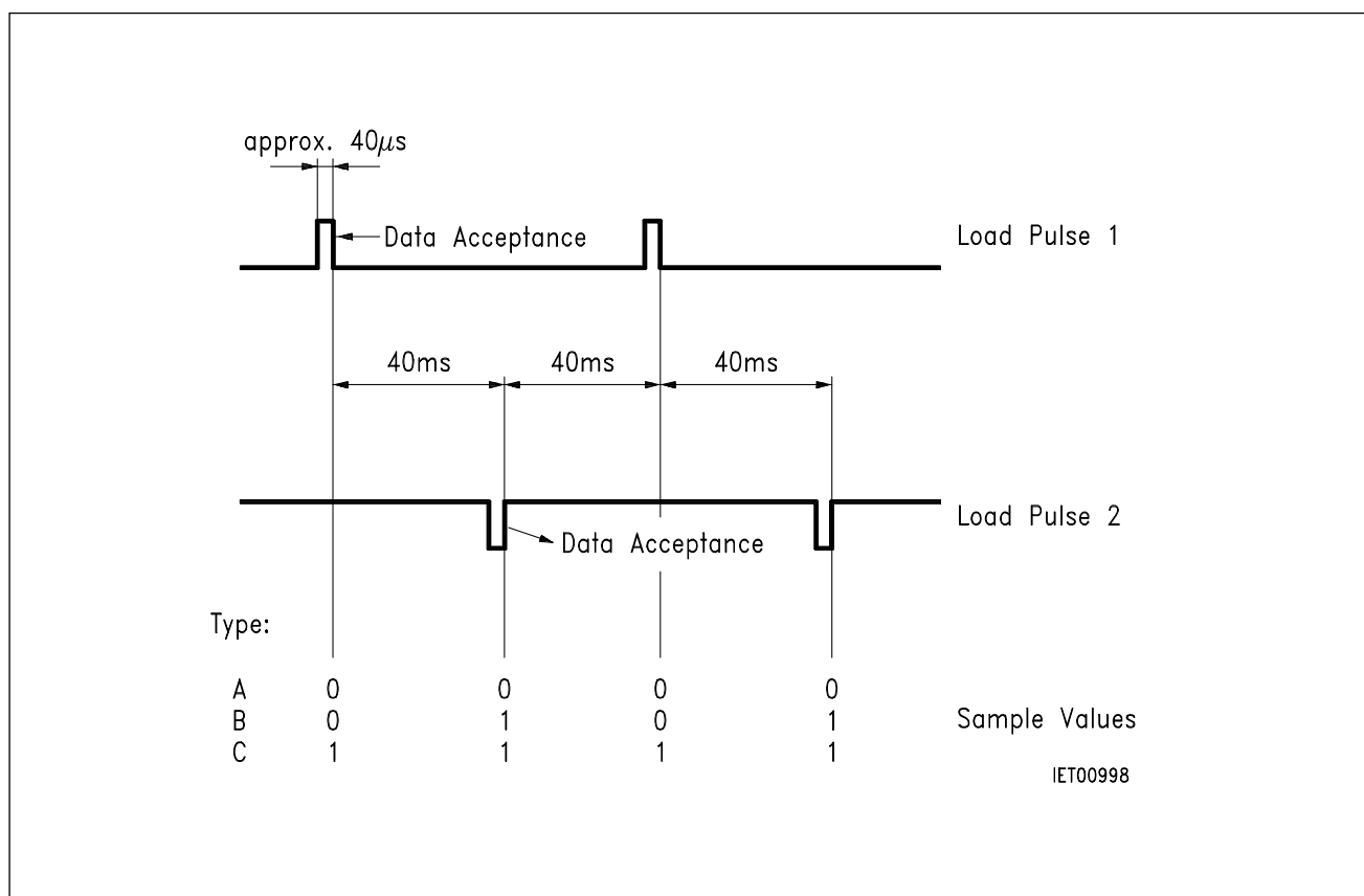
Figure 12 Internal Timing for Distinguishing between the Operating Modes A, B and C
