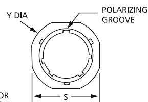
RECEPTACLE ASSEMBLY
