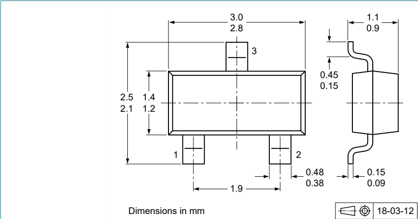
Fig. 11. Package outline SOT23 (TO-236AB)
