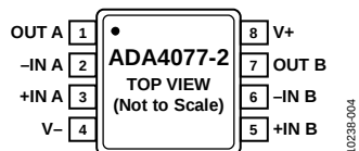
Figure 7. ADA4077-2 Pin Configuration, 8-Lead MSOP
