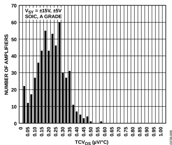
Figure 20. TCV_{OS} Distribution (SOIC, A Grade)
