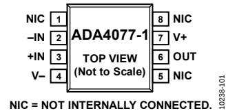
Figure 1. ADA4077-1, 8-Lead SOIC and 8-Lead MSOP
