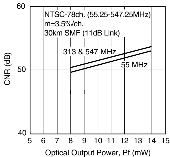
Fig. 12 CNR vs. Output Power
