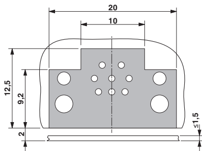
Dimensioned drawing
