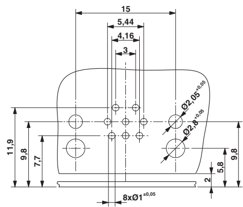
Drilling diagram
