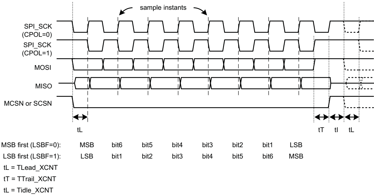
Figure 22-19. SPI Control Timing ( SPICR2[CPHA]=0 , SPICR1[TXEDGE]=1 )
