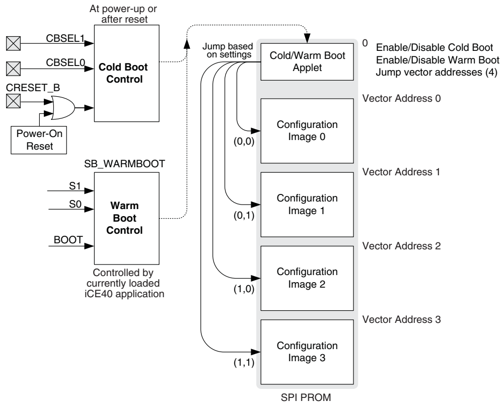
Figure 15-10. Cold Boot and Warm Boot Configuration
