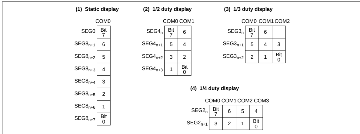
Figure 7 Bit Assignment in an Adn (HD61602)
