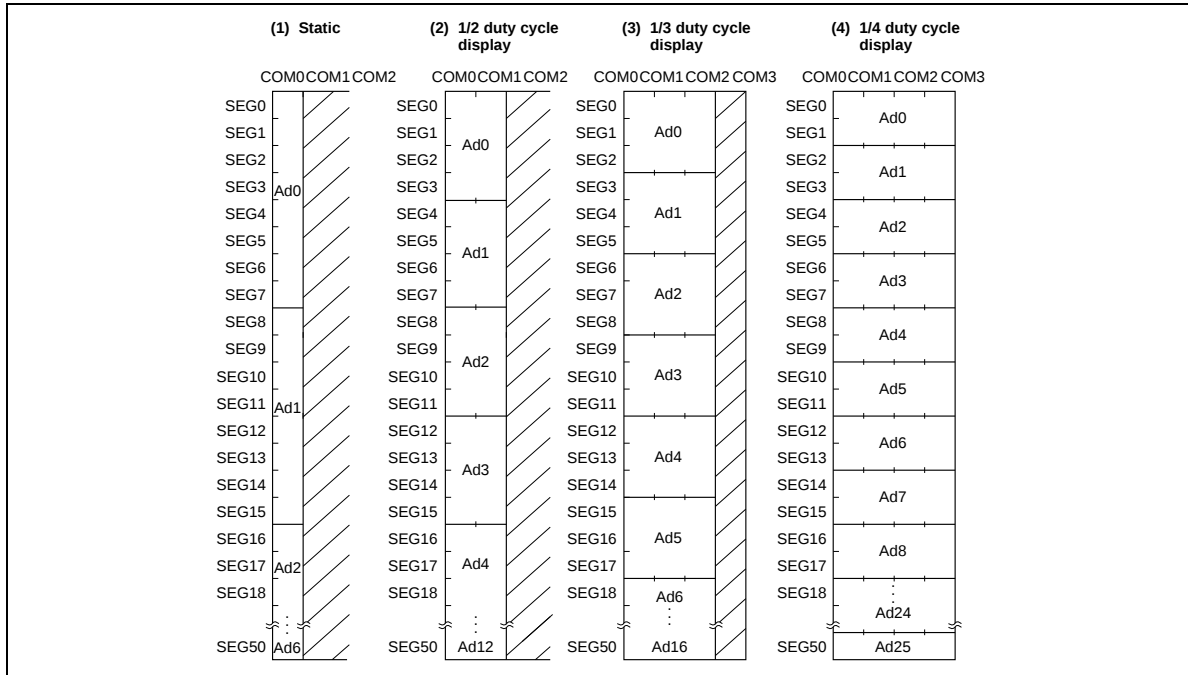
Figure 6 Allocation of Digit (HD61602)
