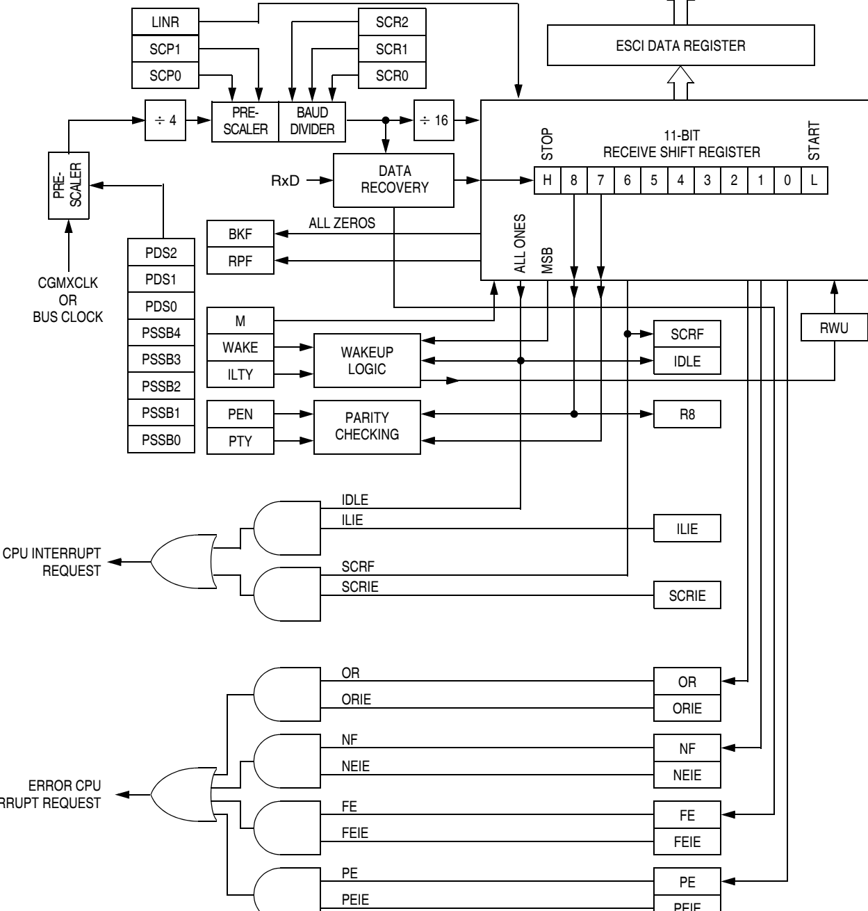
Figure 13-6. ESCI Receiver Block Diagram
