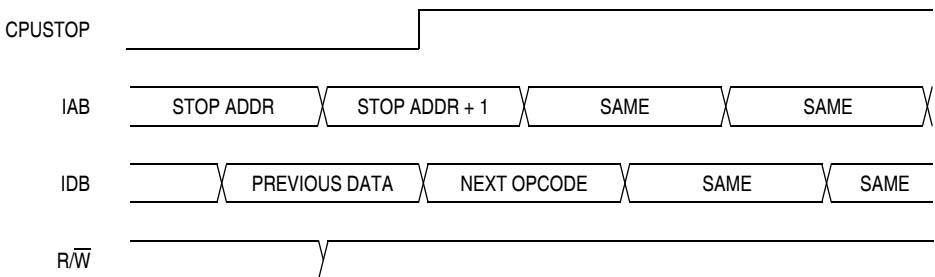
Figure 14-19. Stop Mode Entry Timing
