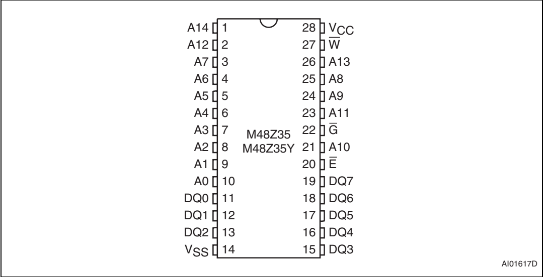
Figure 2. DIP connections
