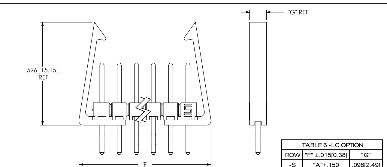
FIG 2 (TSW-1XX-XX-XX-S-LC SHOWN) (SAME AS FIG 1, DIFFERENT AS SHOWN)
