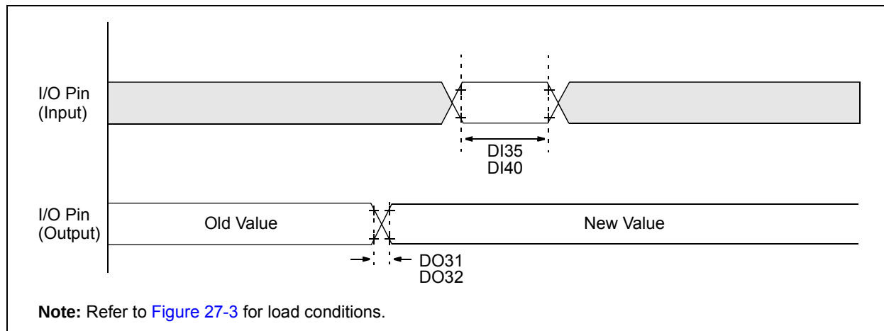
FIGURE 27-5: CLK0 AND I/O TIMING CHARACTERISTICS
