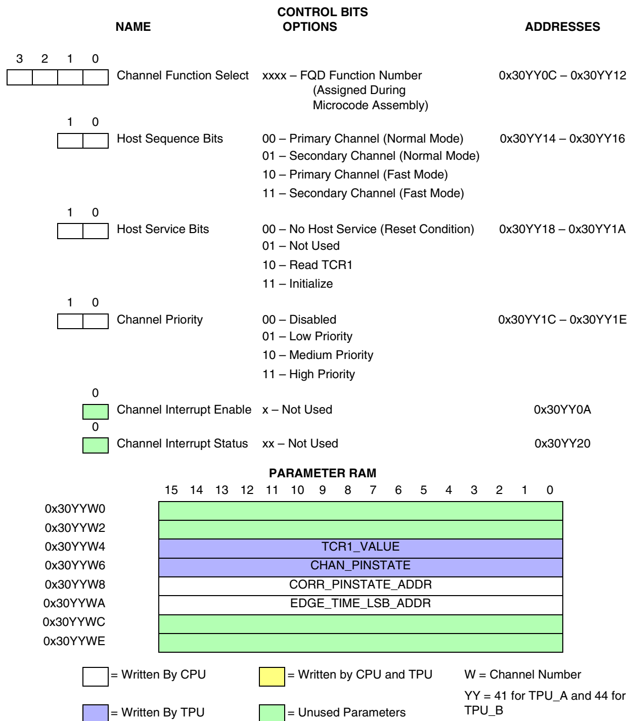
Figure D-20 FQD Parameters — Secondary Channel
