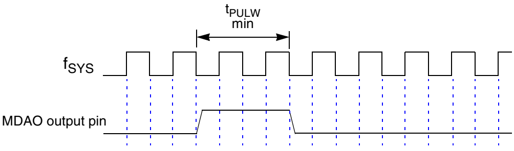
Figure G-47 MDASM Minimum Output Pulse Width Timing Diagram
