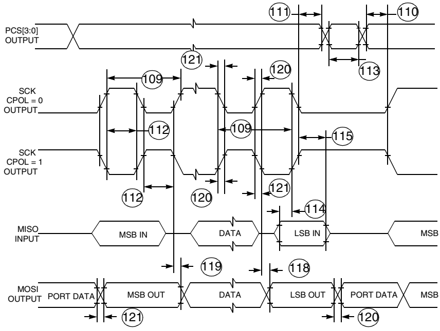
Figure G-30 QSPI Timing — Master, CPHA = 1
