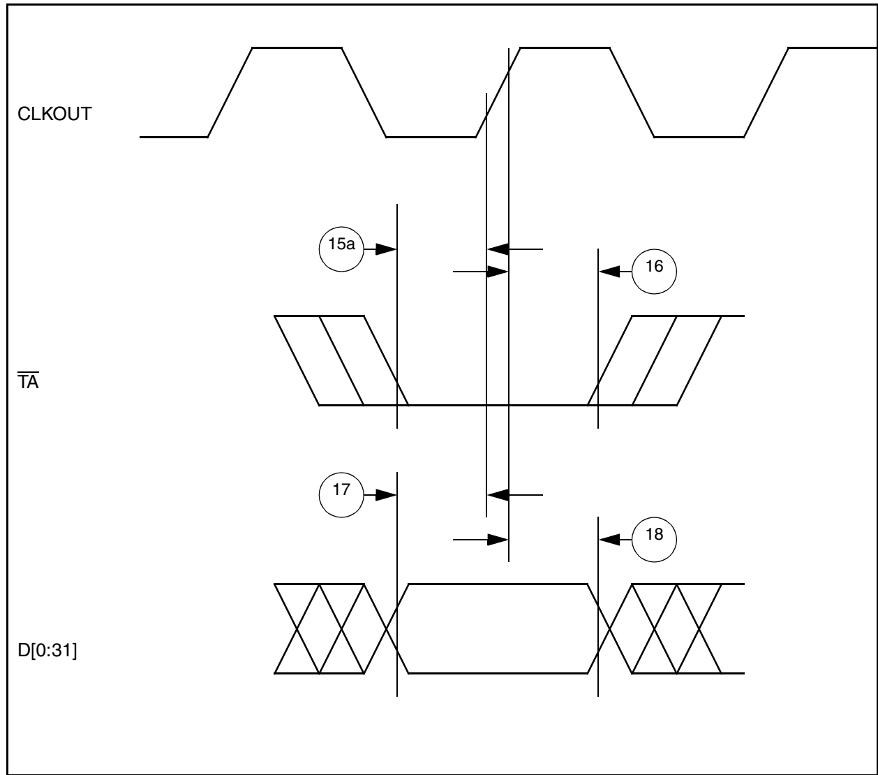
Figure G-6 Input Data Timing in Normal Case
