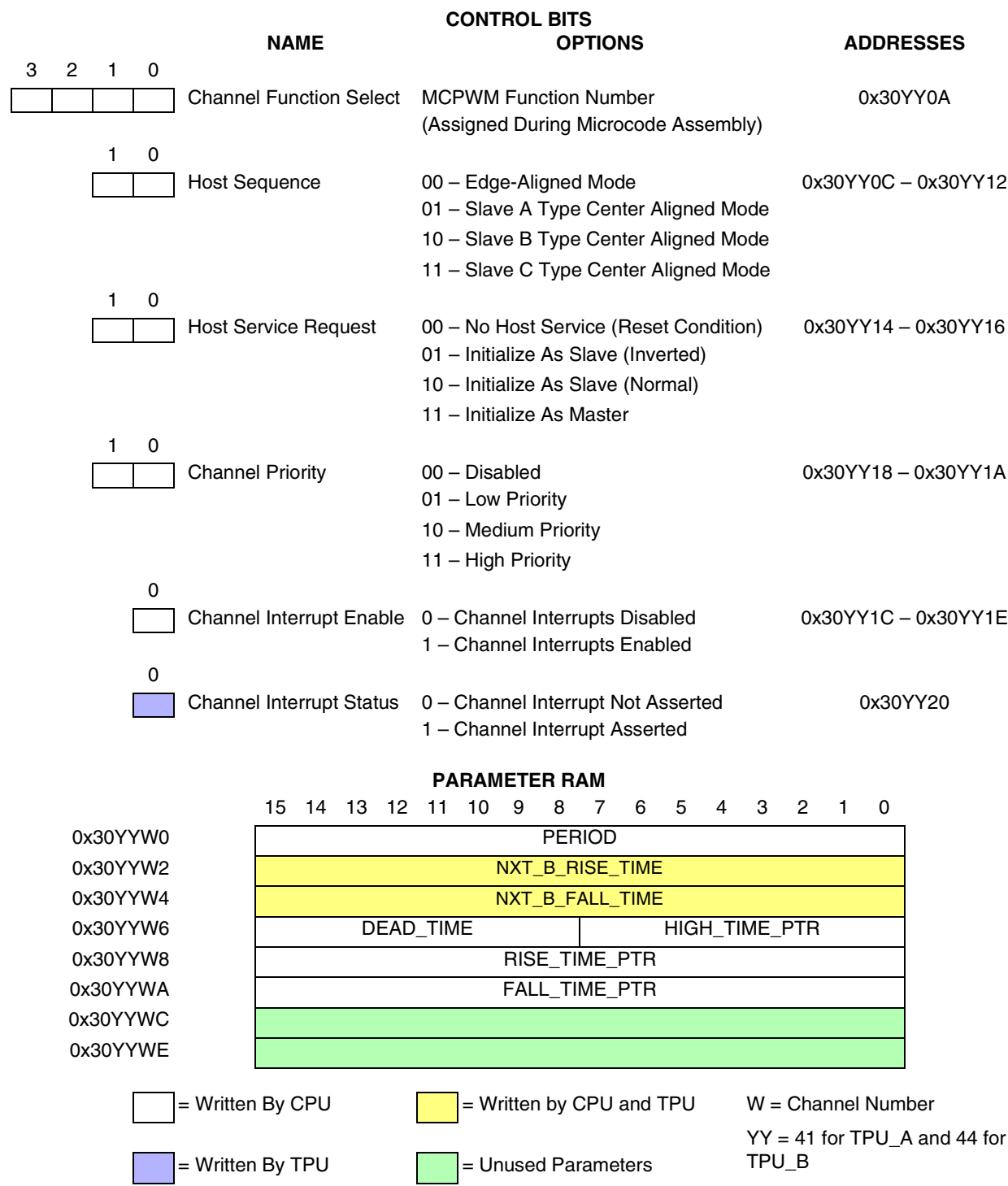
Figure D-15 MCPWM Parameters — Slave Ch A Non-Inverted Center-Aligned Mode
