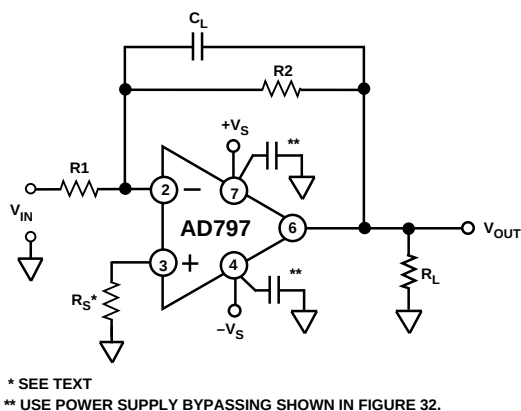
Figure 37. Inverting Amplifier Connection
