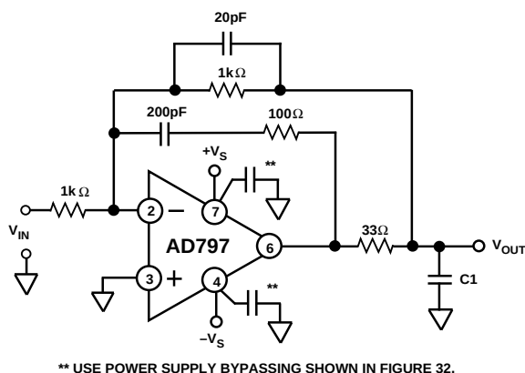
Figure 39. Recommended Circuit for Driving a High Capacitance Load
