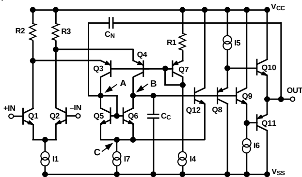
Figure 27. Model of AD797 vs. That of a Typical Three-Stage Amplifier
