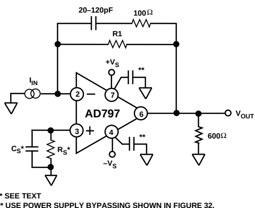
Figure 36. I-to-V Converter Connection
