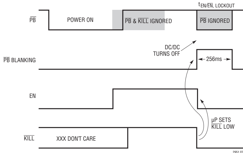
Figure 4. DC/DC Turn-Off Blanking (LTC2951-1)
