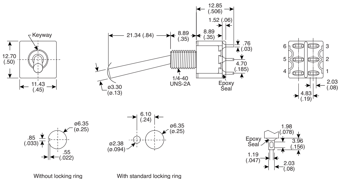
Panel Mounting
