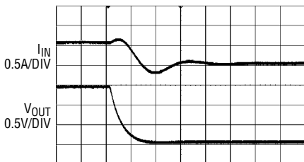
Short-Circuit with 4A Load
