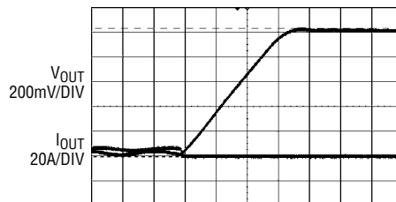
Recovery to No Load from Short Circuit
