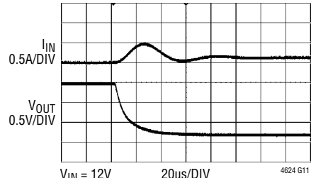
Short-Circuit with No Load
