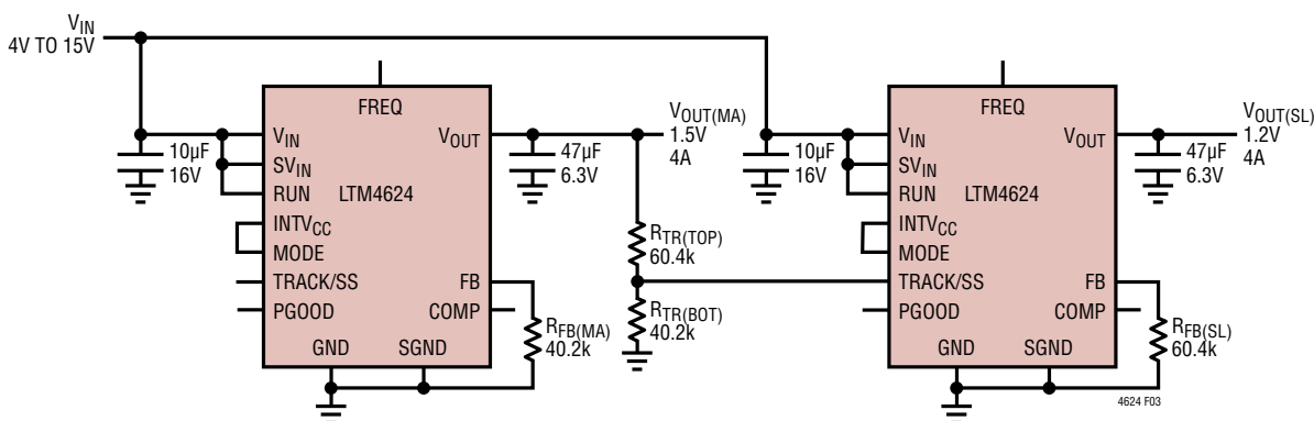
Figure 3. Example Schematic of Ratiometric Output Voltage Tracking
