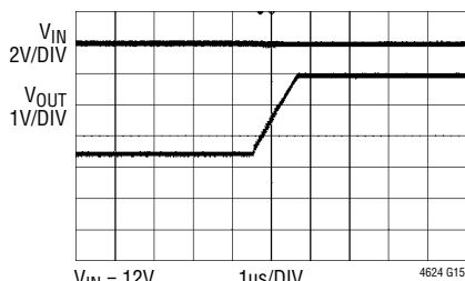
Start Into Pre-Bias Output
