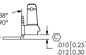
IN-PROCESS SCALE 8:1 (AUTOMATED ONLY)
