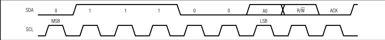
Figure 3. Slave Address
